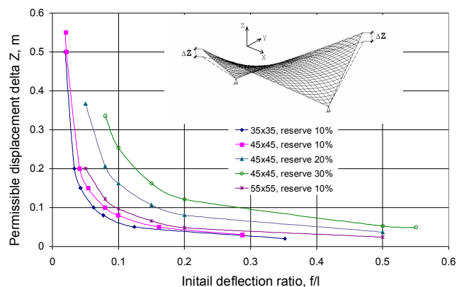
Fig 3. Permissible displacements of supports of primary element depending on initial deflection of primary element
